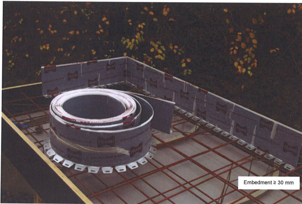
Coated metal water stop " FraDiflex Premium with mounting angle" - double side coated – for horizontal construction joints
