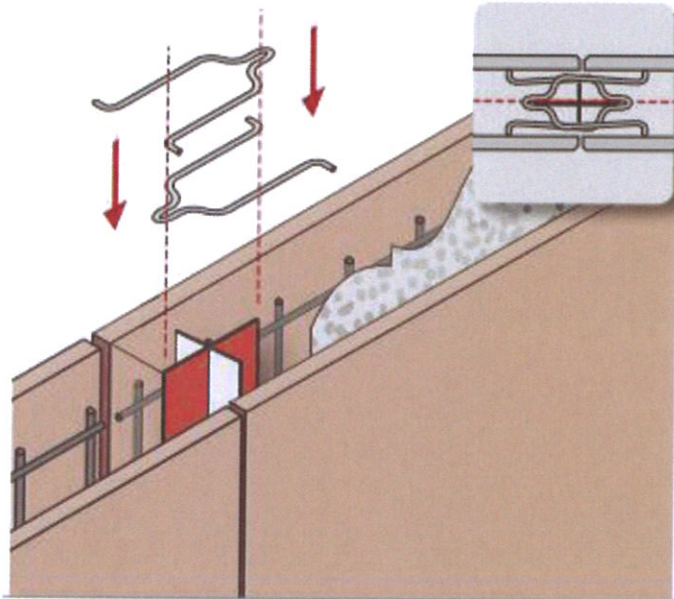
Fradiflex Stremaflex Stop end panel
